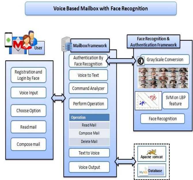
Figure: System Architecture of Proposed System
