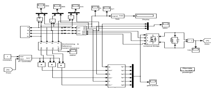
Fig. 6. Simulated power circuit for PI controlled improved power quality converter
