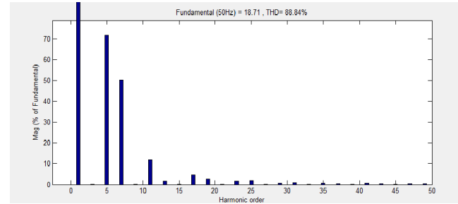
Fig. 9 Harmonics spectrum without controller
