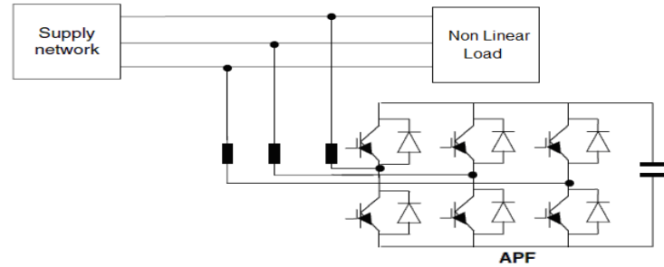
Fig. 1: Active power filter connected with transmission line
