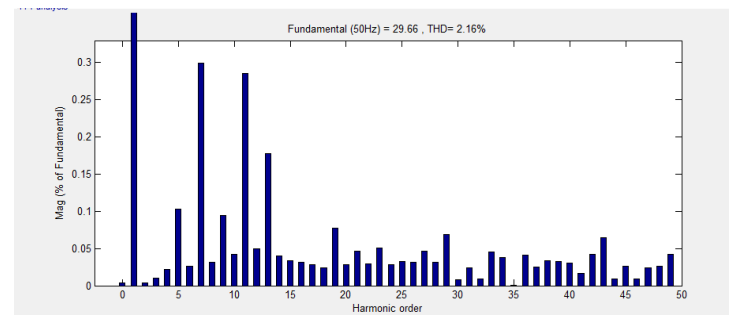
Fig. 10 Harmonics spectrum with PI controller
