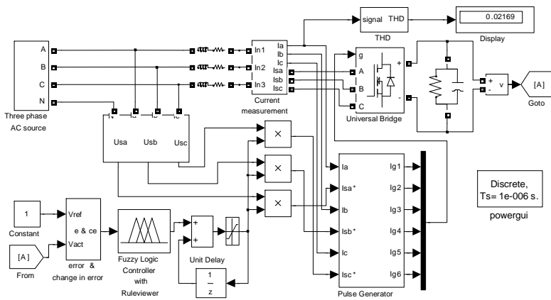
Fig. 7. Simulated power circuit for Fuzzy controlled improved power quality converter
