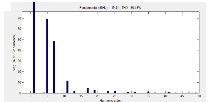
Fig. 10 Harmonics spectrum with PI controller
