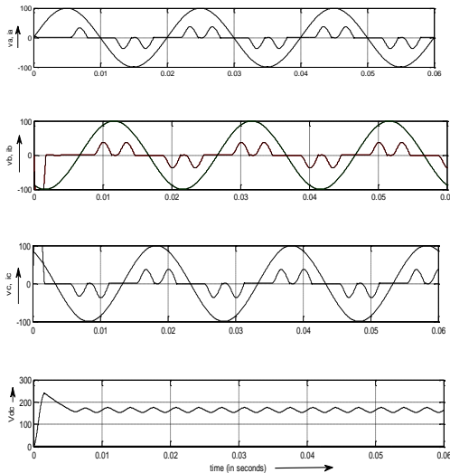
Fig. 8 Waveform without controller
