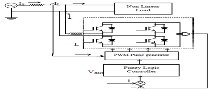
Fig. 4 Block Diagram of Fuzzy controlled improved power quality converter
